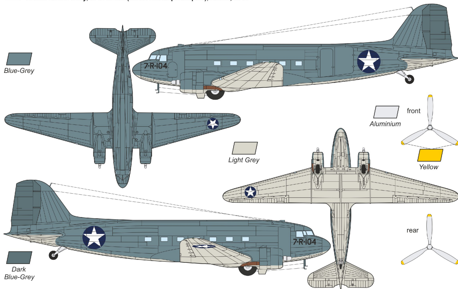
B Douglas R4D-1 Skytrain (DC-3A-360), 7-R-104 (BuNo unknown), Transport Squadron 7 (VR-7), Naval Air Transport Service (NATS), United States Navy, NAS Miami (Miami Municipal Airport), U.S.A., 1943
