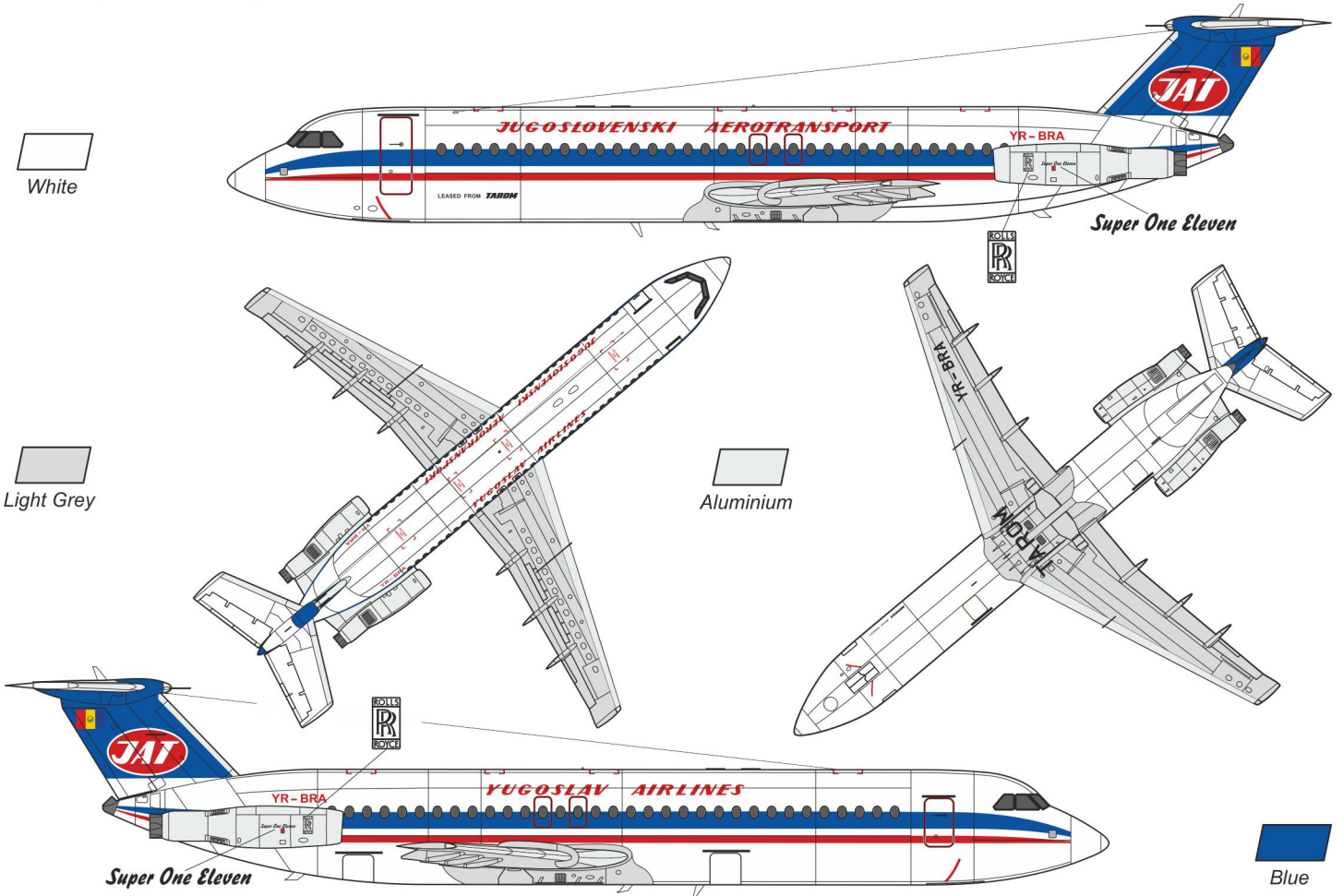
C Rombac (BAC) 1-11-500 (561RC), YR-BRA (c/n 401), JAT Yugoslav Airlines/Jugoslovenski Aerotransport (a/c leased from Tarom), Belgrade Airport, Yugoslavia, 1989
