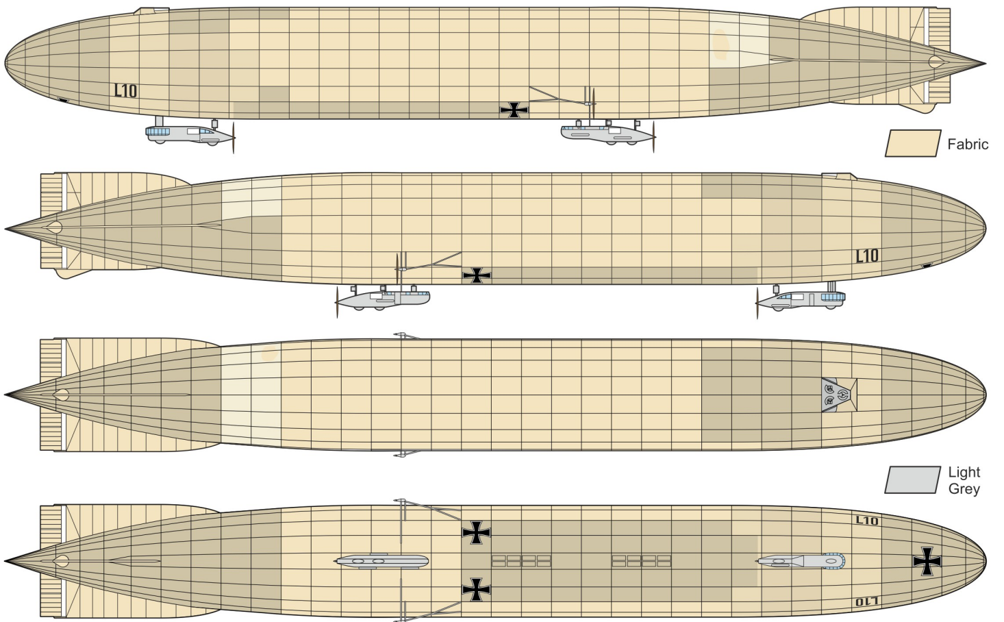
B Zeppelin LZ40 (P-class), L10, Black L10, Naval Airship Division (Marine-Luftschiff-Abteilung), Imperial German Navy (Kaiserliche Marine), Hage Airship Base, Germany, summer 1915
